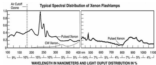
Figure 2. Typical spectral output of a Xenon flashlamp (Sonenshein, 2003).
